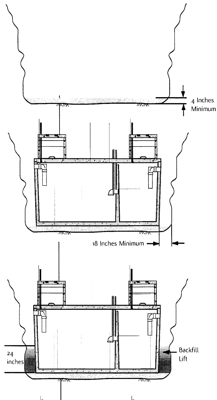
Figure 3 — Basic principles of bedding, tank placement and backfilling
